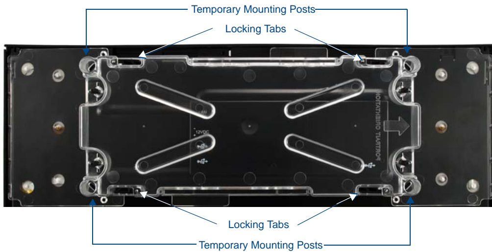
FIG. 14 MXD-1900L-PAN Back Box
