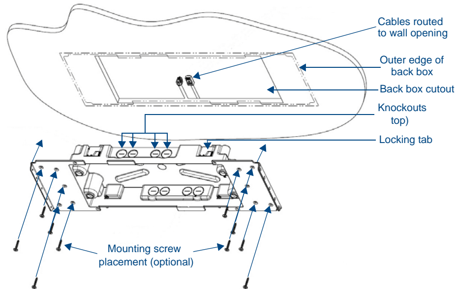
FIG. 18 MXD-1900L-PAN Back Box installation (Landscape)
