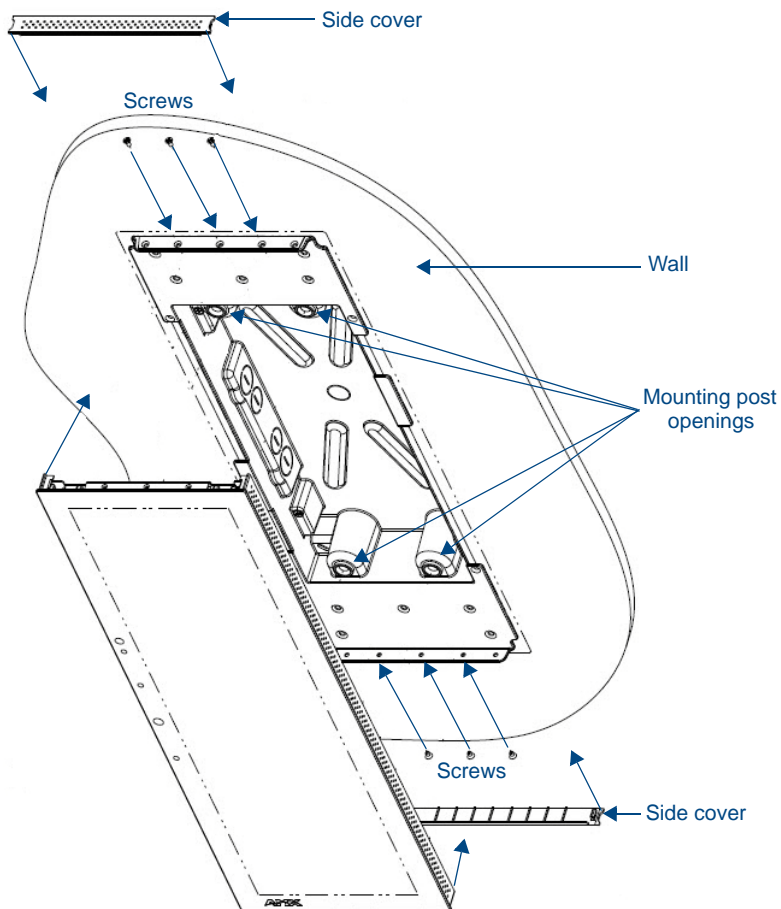
FIG. 22 MXD-1900L-PAN installation (Portrait)
