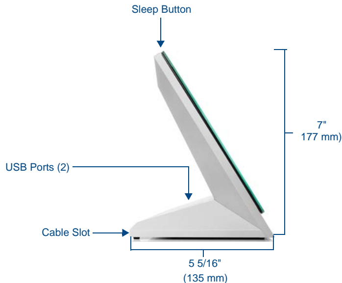
FIG. 2 MXT-1900L-PAN side view
