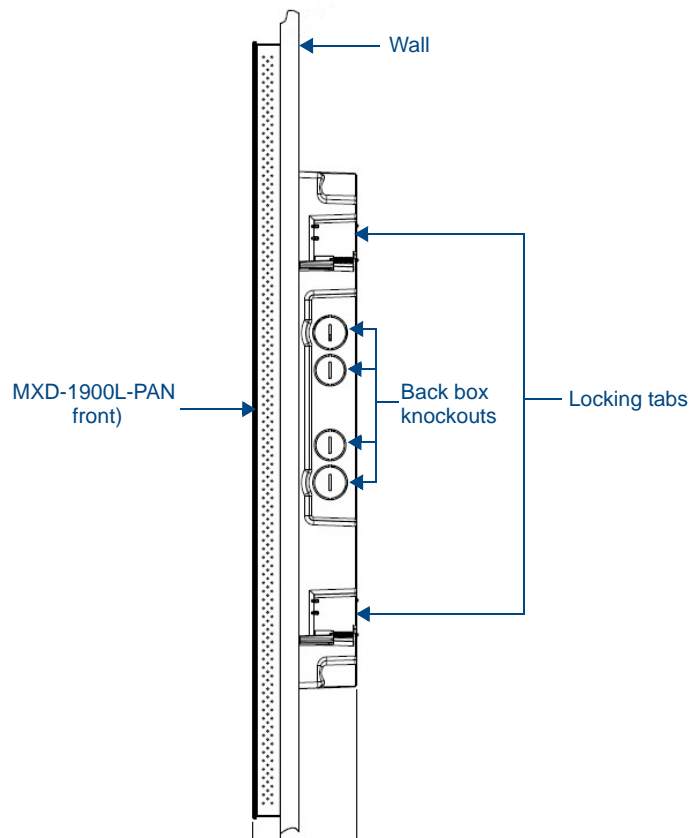
FIG. 16 Side view of installed MXD-1900L-PAN (Portrait)
