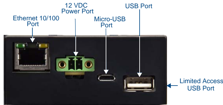
FIG. 20 MXD-1900L-PAN rear connectors (front view)
