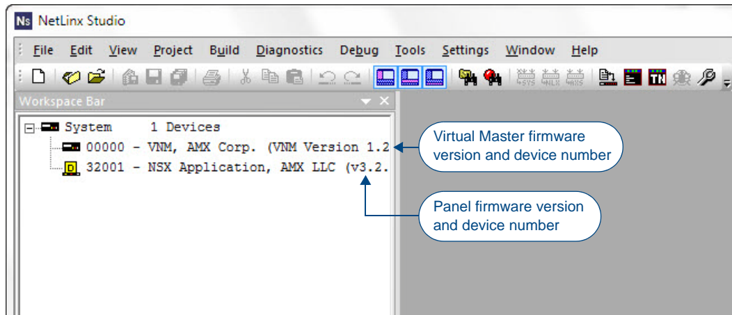
FIG. 32 NetLinx Workspace window (showing panel connection via a Virtual NetLinx Master)
