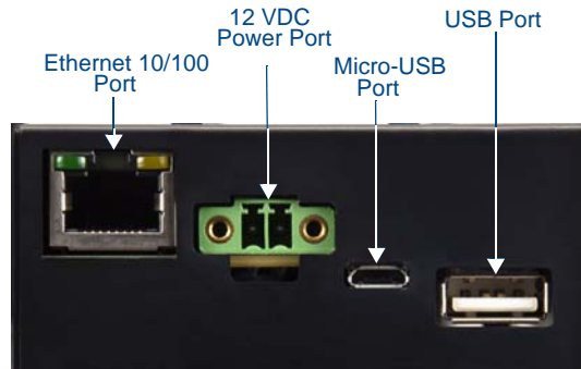
FIG. 9 MXT-1900L-PAN underside connectors
