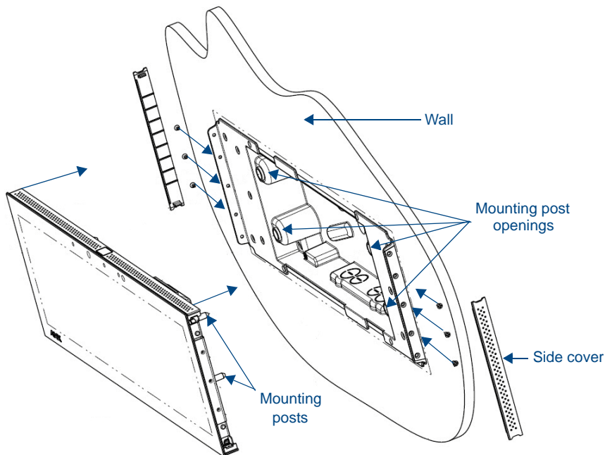
FIG. 21 MXD-1900L-PAN installation (Landscape)
