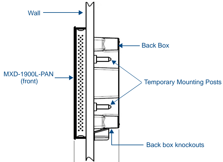
FIG. 15 Side view of installed MXD-1900L-PAN (Landscape)
