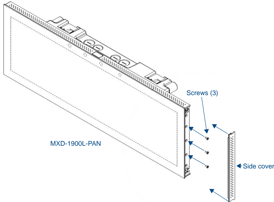
FIG. 23 MXD-1900L-PAN side cover installation (Landscape)
