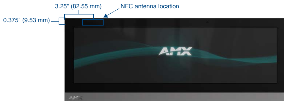
FIG. 8 NFC antenna location on the MXT-1900L-PAN
