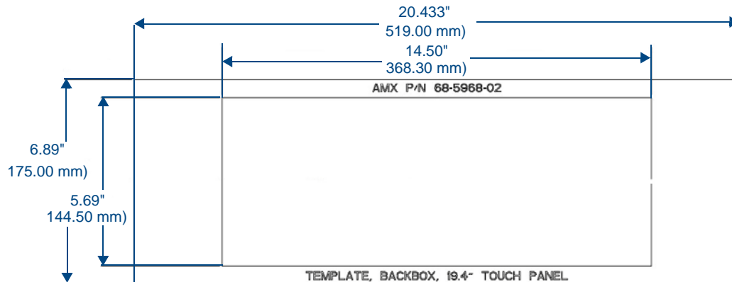
FIG. 17 MXD-1900L-PAN Template
