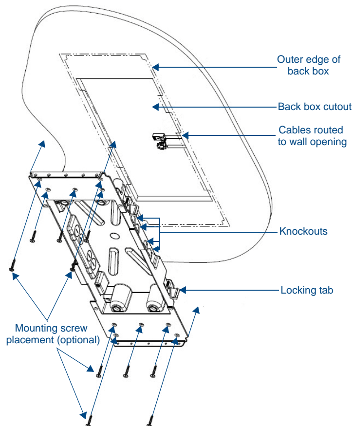
FIG. 19 MXD-1900L-PAN Back Box installation (Portrait)
