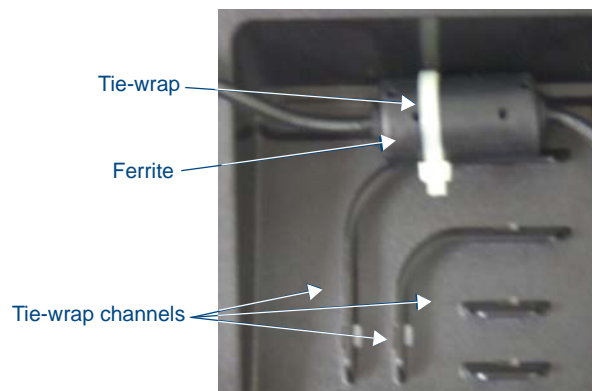
FIG. 10 Tie-wrap for power connector ferrite
